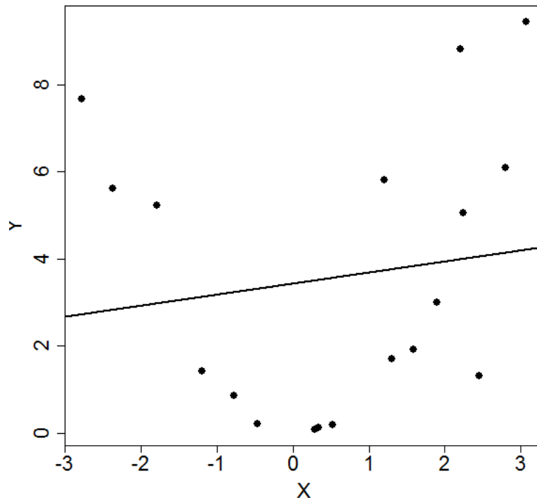
Figure 1.2: The insertion of an irrelevant regression line through the scatter of points alludes to the existence a linear relationship.
