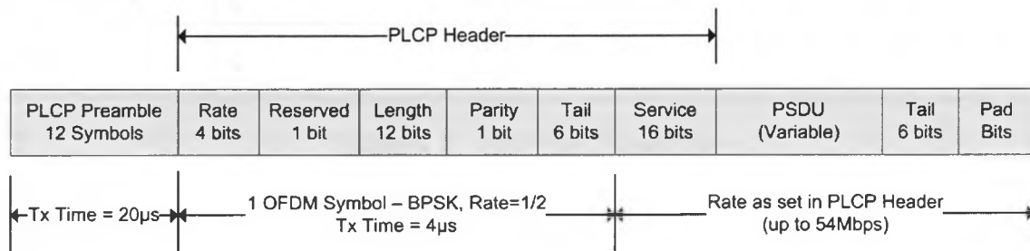
Figure 4.5: 802.11a Packet
