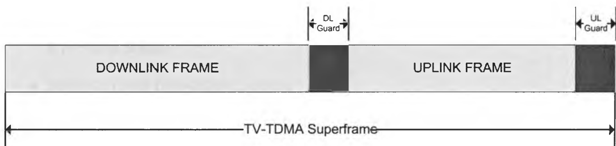
Figure 4.2: TV-TDMA Superframe
