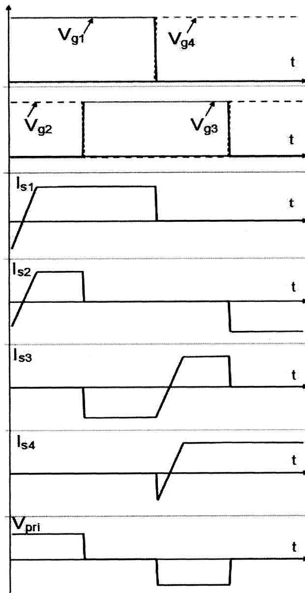
Figure 1.8: Typical dc-dc full-bridge waveforms.
