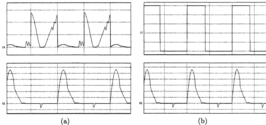
Figure 5.4: Simulated waveforms of (a) ZCS switch voltage (top) and switch current (bottom) [V: 250V/div, I: 5A/div, t: 5 \mu s/div]. (b) Gate pulse (top) and switch current (bottom) [V: 5V/div, I: 10A/div, t: 5 \mu s/div].
