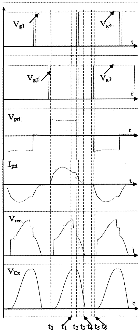
Figure 2.8: Steady state waveforms of dc-dc ZVZCS full bridge PWM converter.
