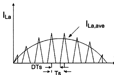
Figure 1.12: Input line current waveform of a three-phase ac-dc single-switch boost converter (half-line cycle).
