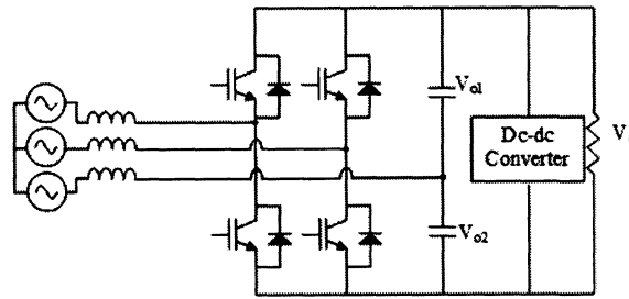
Figure 1.10: Three-phase ac-dc converter with four switches.
