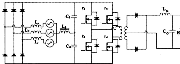
(b) Compromising between voltage regulation and PFC ([6])
