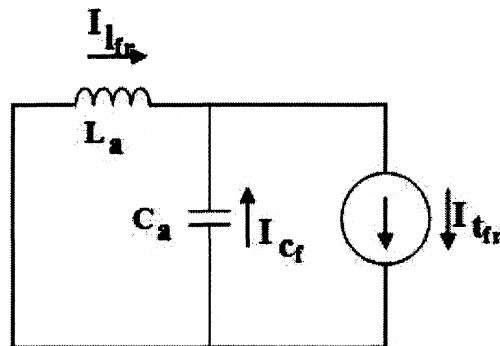
Figure 4.9: Single-phase equivalent input filter diagram.
