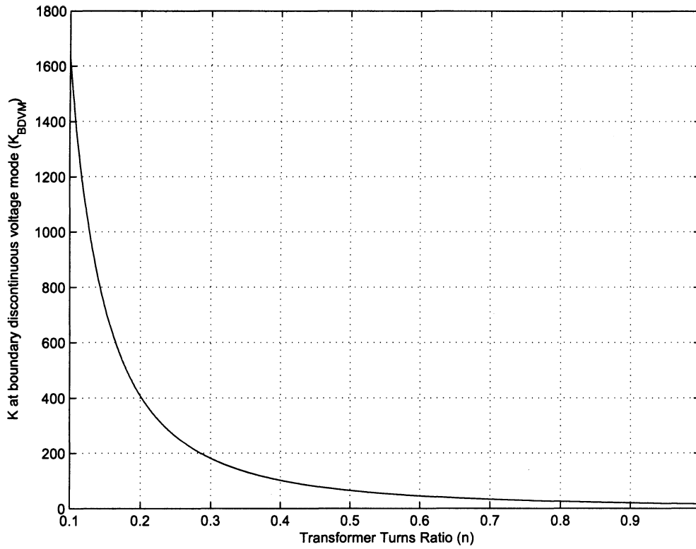
Figure 4.8: K_{BDVM} vs. n for BDVM operation.
