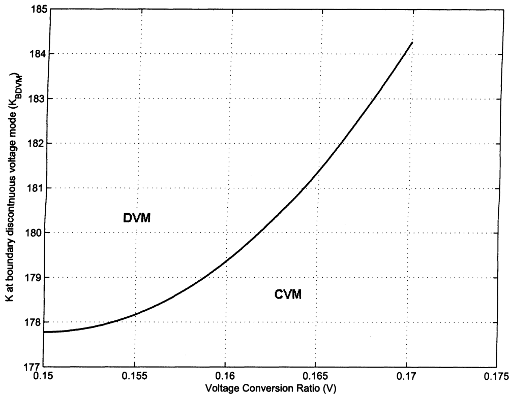
Figure 4.6: The curve of K^{BDVM} vs. V^{BDVM} .
