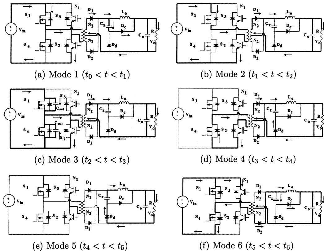
Figure 2.7: Modes of operation of dc-dc ZVZCS full bridge PWM converter.
