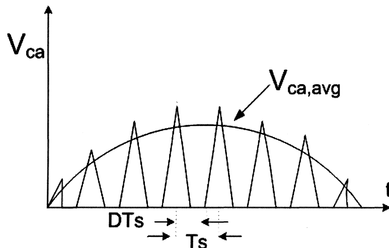
Figure 5.1: Triangular input capacitor voltage and sinusoidal envelope.
