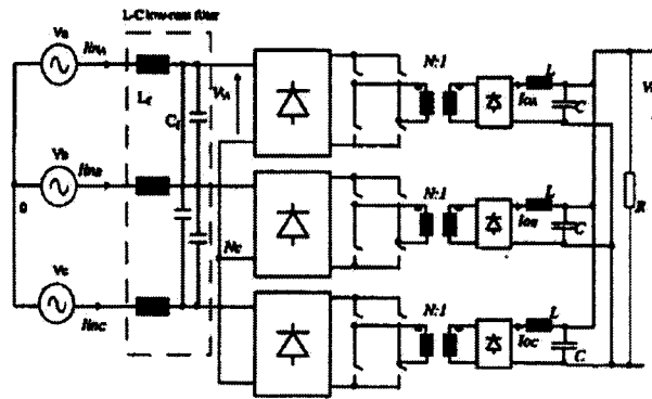
(a) Converter with three single-phase modules ([13])
