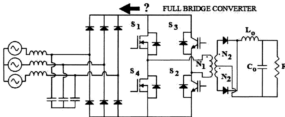
Figure 2.5: Three-phase single-stage ac-dc converter with conventional full-bridge.
