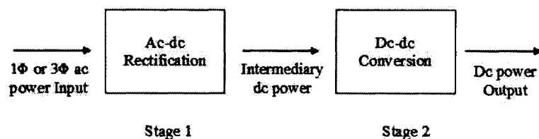
Figure 1.5: Block diagram of Two-Stage ac-dc converters.
