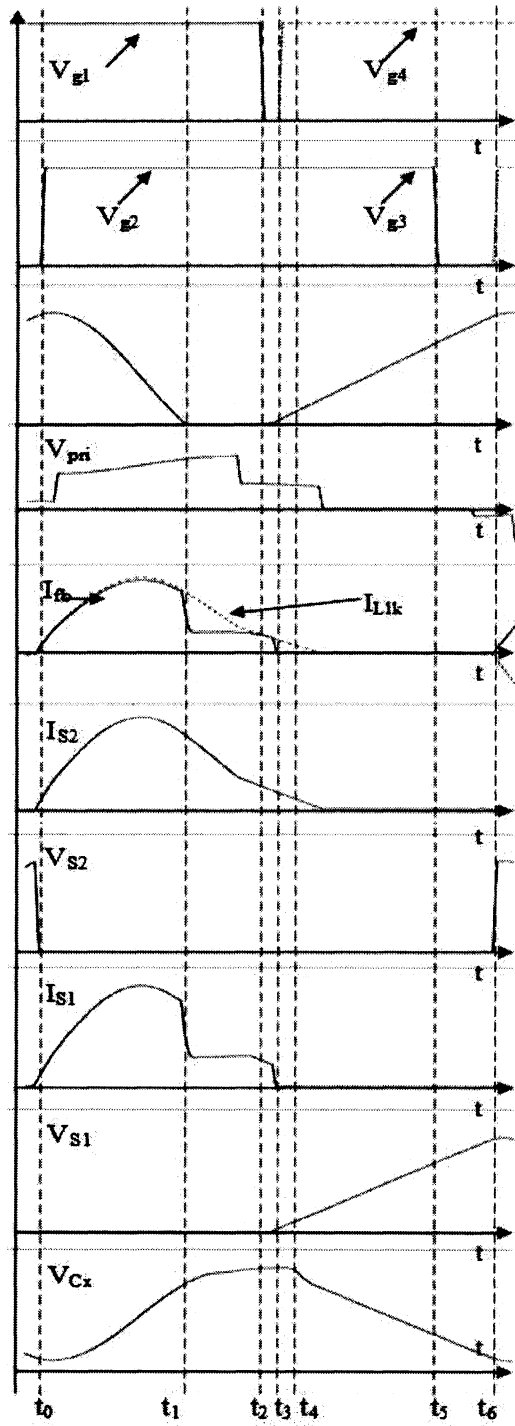
Figure 3.4: Proposed converter typical waveforms.
