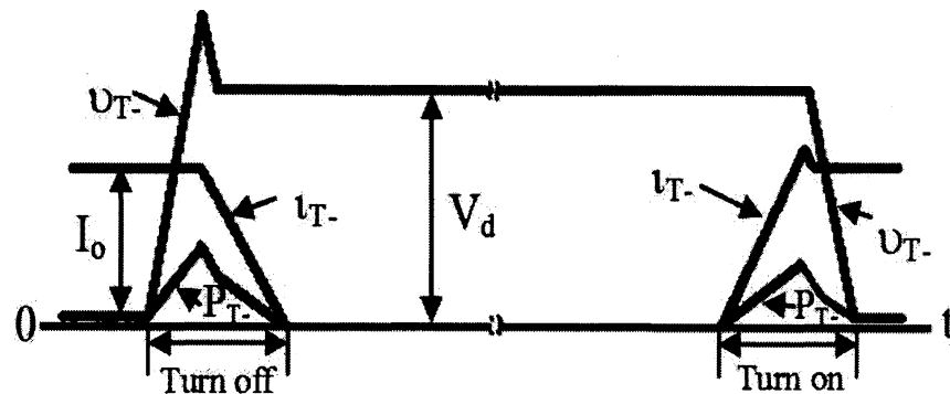
Figure 1.4: Non-ideal switching characteristics of a semiconductor device.
