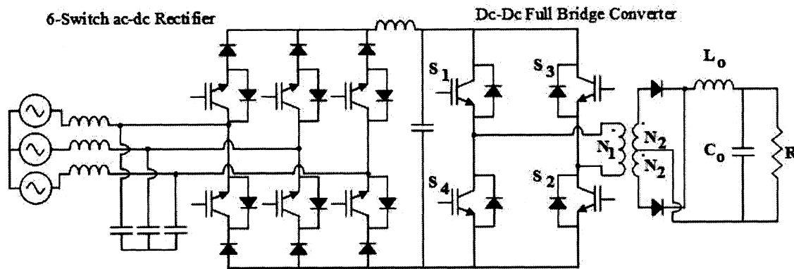
Figure 1.6: Three-phase ac-dc six switch two-stage full-bridge converter.
