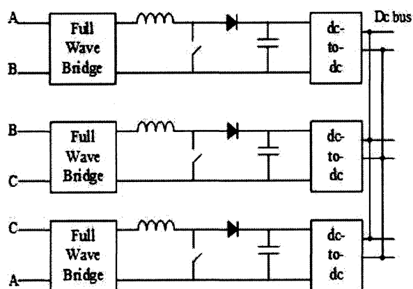
Figure 1.9: Three-phase ac-dc converter using three single-phase modules.
