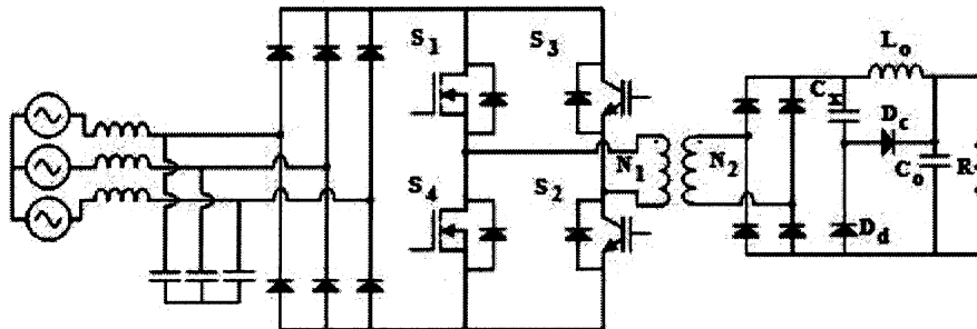
Figure 3.1: Proposed three-phase single-stage ac-dc converter with ZVZCS full-bridge.
