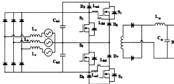
(c) A multi-level converter ([10])
