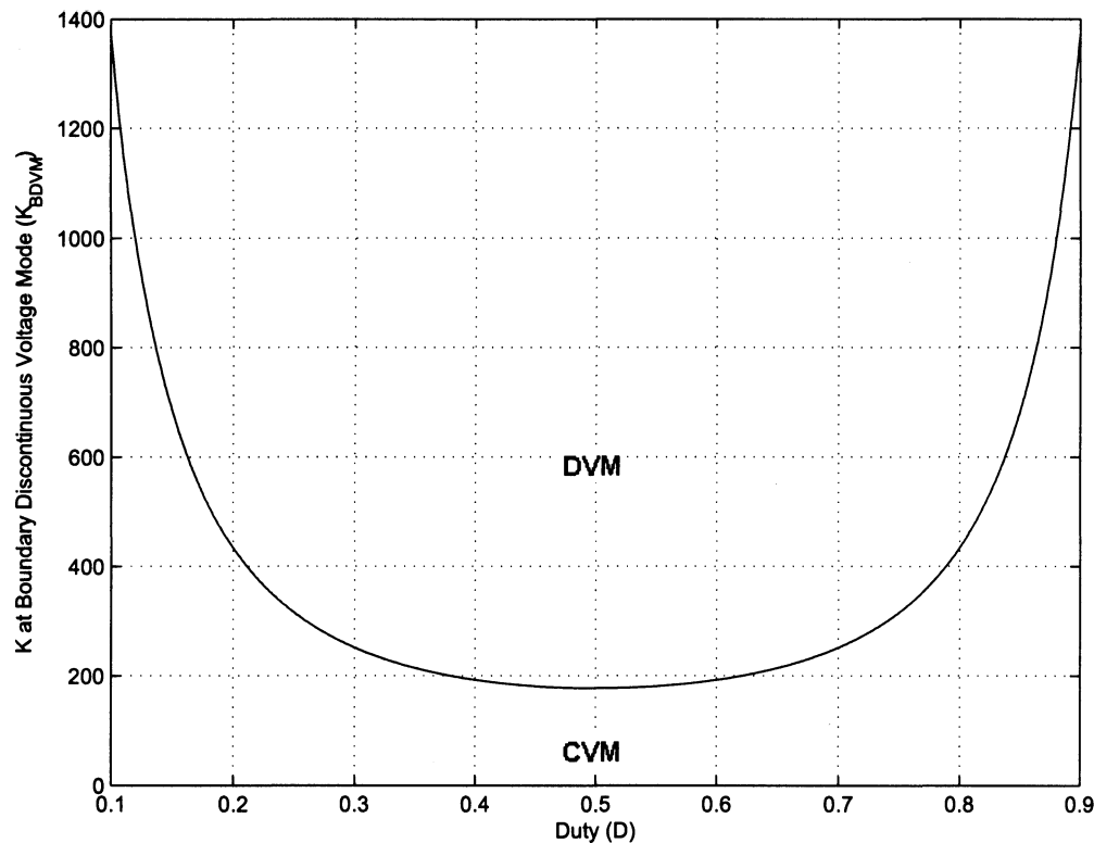
Figure 4.7: K_{BDVM} vs. D-K_{BDVM} for BDVM operation for the selected duty range.
