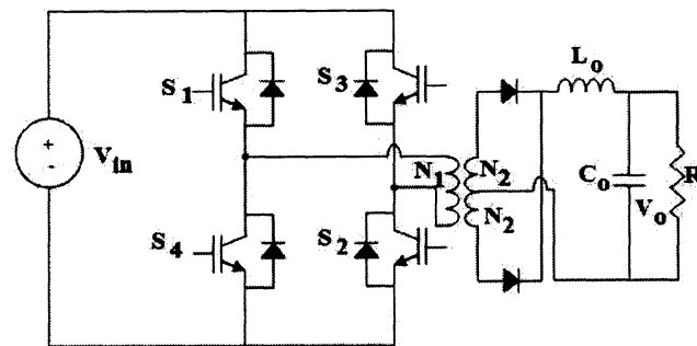
Figure 1.7: Dc-dc full-bridge converter.
