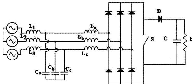
Figure 1.11: Three-phase ac-dc single-switch PFC front-end boost converter.
