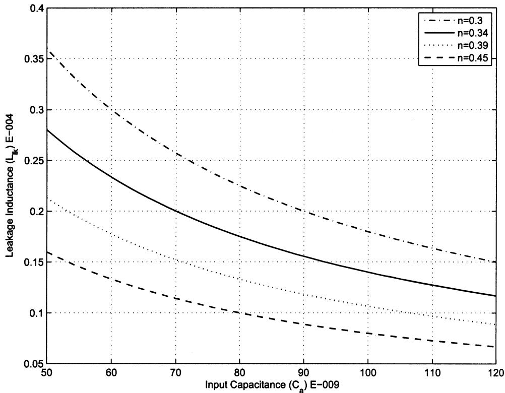
Figure 4.10: Curves of L_{lk} vs. C_a for different values of n .
