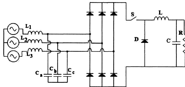
Figure 1.13: Three-phase ac-dc single-switch PFC front-end buck converter.
