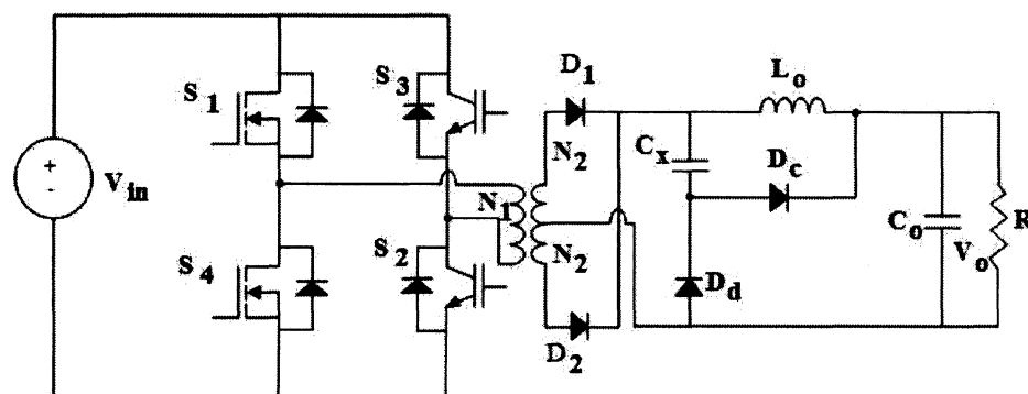
Figure 2.6: Dc-dc PWM ZVZCS full-bridge converter.
