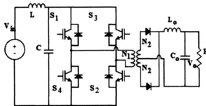
Figure 4.2: Dc-dc full bridge converter with L-C filter.
