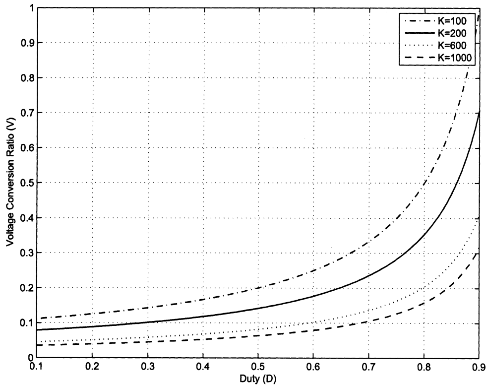
Figure 4.5: V vs. D for selected K values.
