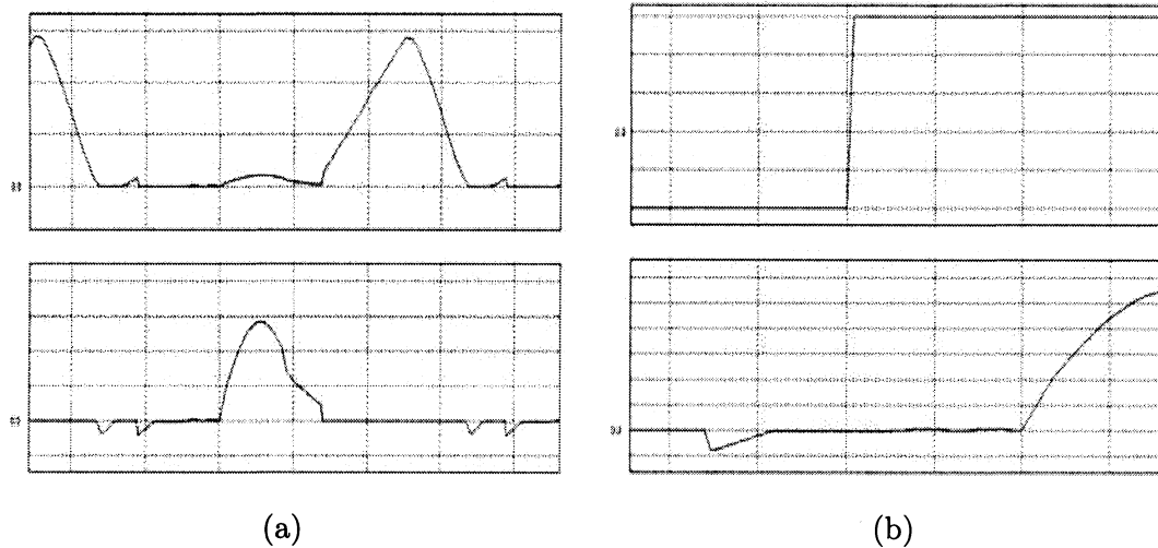
Figure 5.2: Simulation results of typical (a) ZVS switch voltage (top) and switch current (bottom) [V: 250V/div, I: 10A/div, t: 5 \mu s/div], (b) Gate pulse (top) and switch current (bottom) [V: 5V/div, I: 10A/div, t: 1 \mu s/div].
