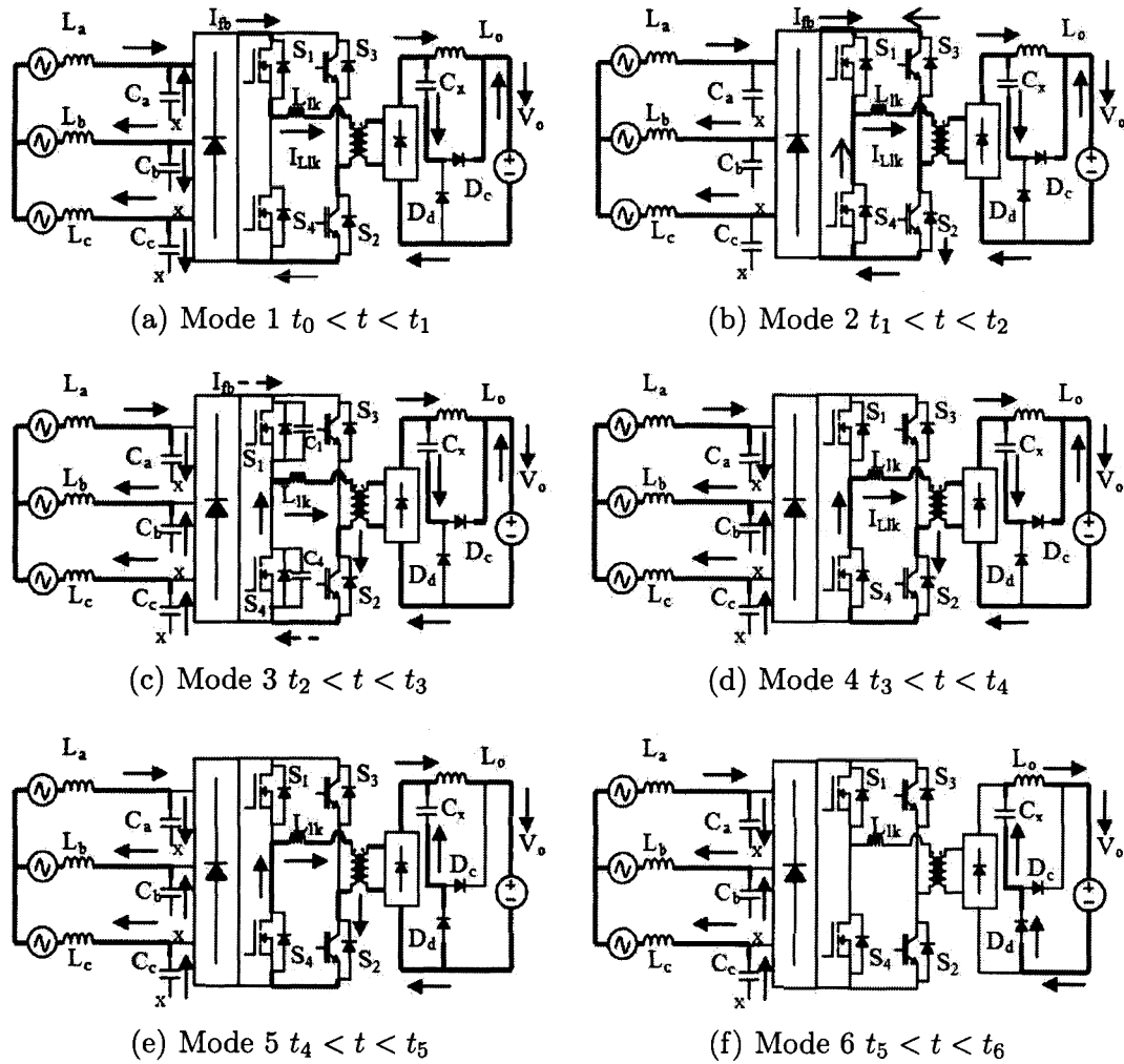
Figure 3.3: Modes of converter operation.
