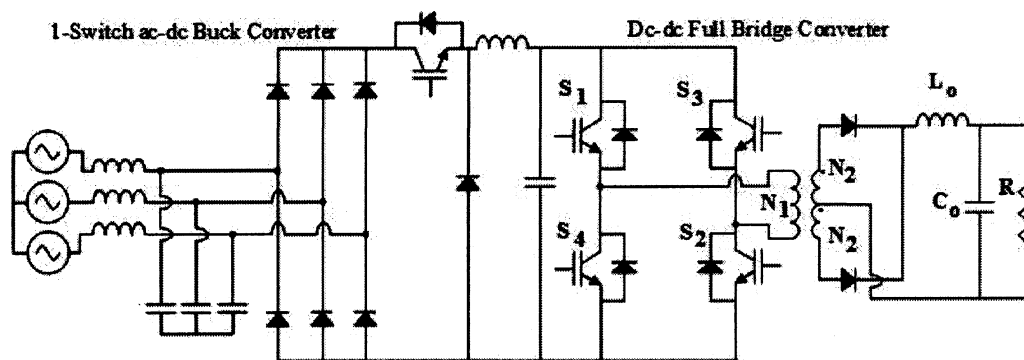
Figure 2.1: Ac-dc converter with single-switch buck rectifier and dc-dc full-bridge converter.
