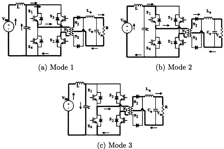
Figure 4.3: Steady state modes of operation of the single-phase equivalent circuit.
