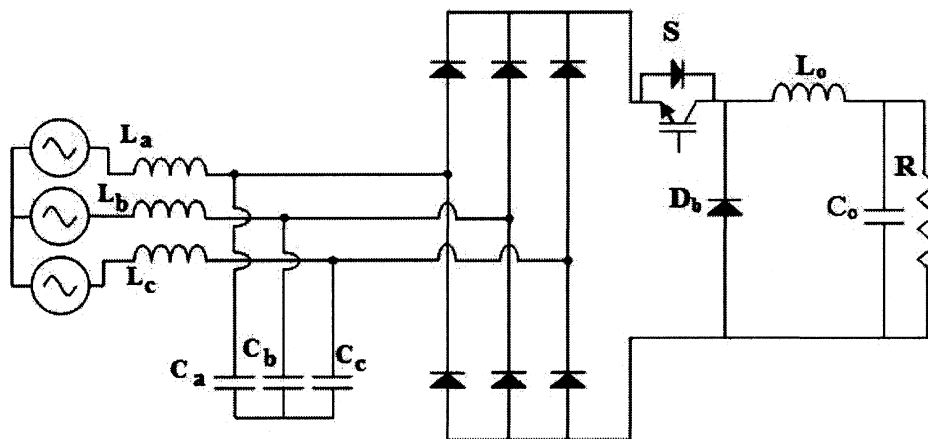
Figure 2.2: Three-phase ac-dc single-switch PFC buck converter.
