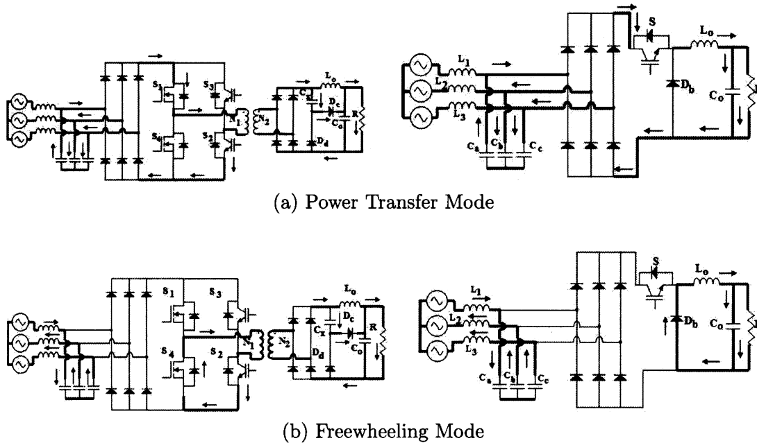
Figure 3.2: Comparison of the proposed converter to a three-phase single switch buck converter.
