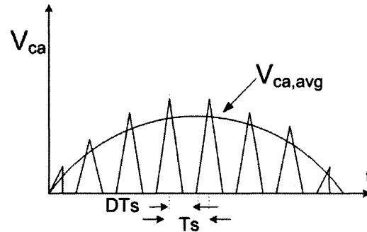
Figure 2.4: Input capacitor voltage of a three-phase, single-switch, ac-dc buck converter (half-line cycle).
