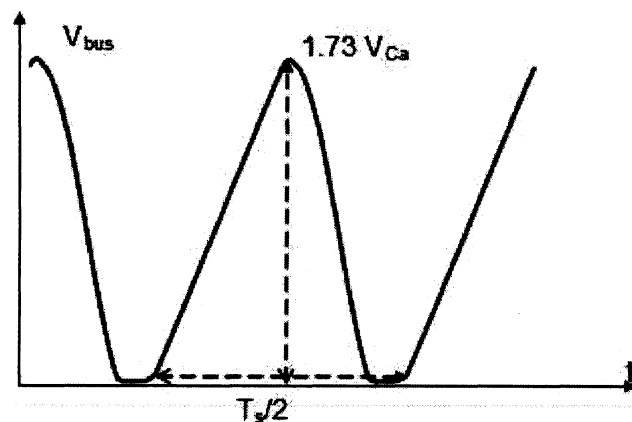
Figure 4.1: Bus voltage of the proposed converter when input capacitors in DVM.
