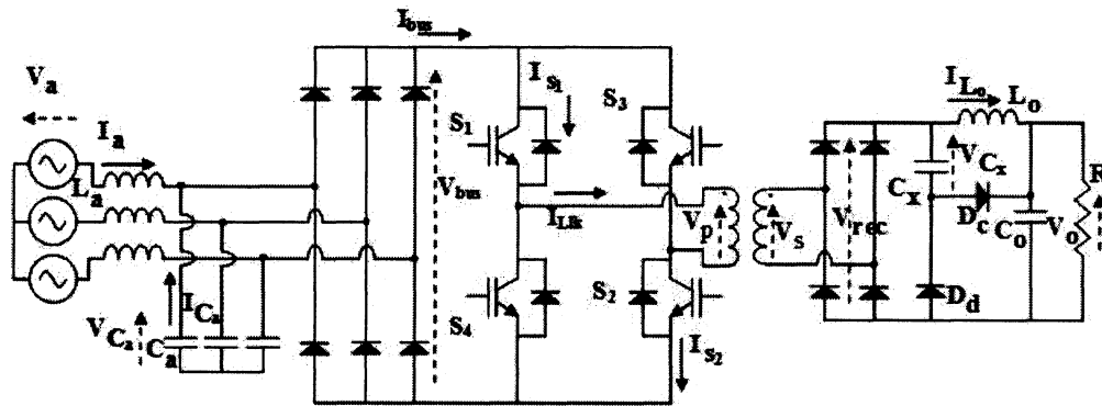
Figure 4.4: Proposed converter.
