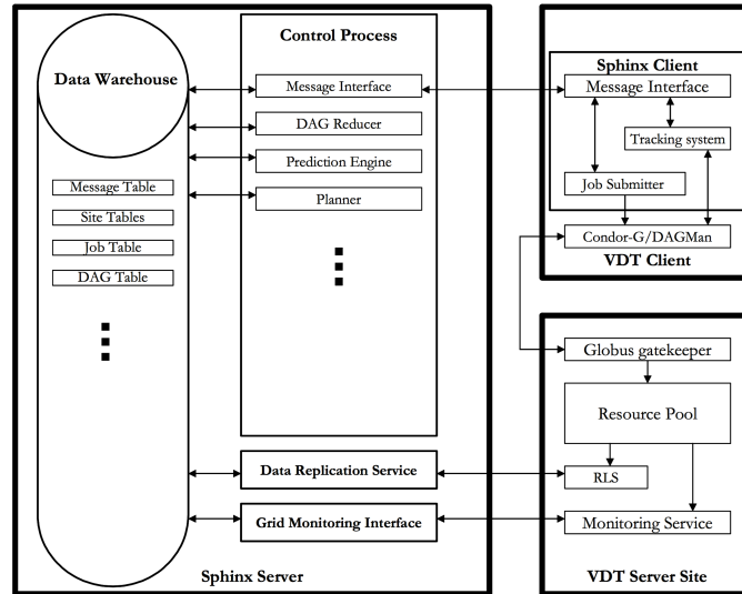
Figure 2-1: The Sphinx Scheduling System [44]
