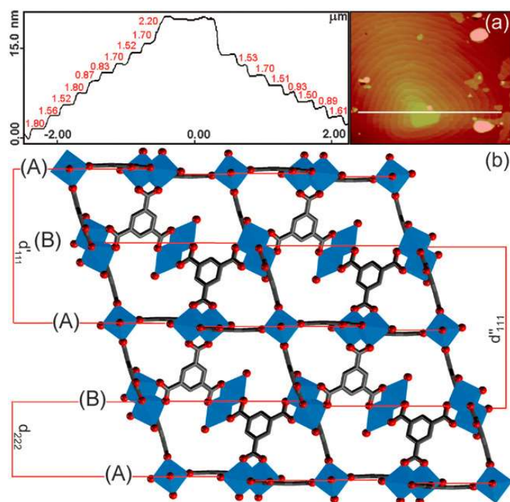
Figure 1-6 Cross-sectional analysis of a typical step train on the \{111\} face of HKUST-1 (a) and the structure of HKUST-1 viewed down a [110] direction highlighting possible d_{111} and d_{222} crystal spacings (b). 36
