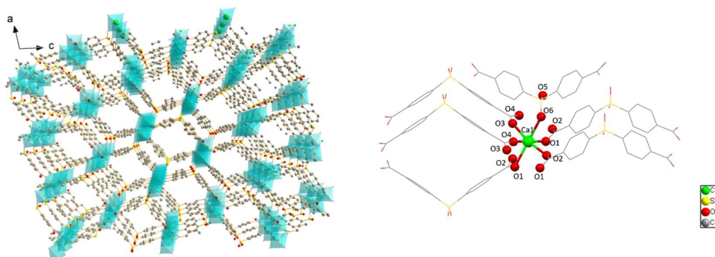
Figure 4-3 (Left) structure of CaSDB viewed along b axis; (Right) Local structure and Calcium coordination environment of CaSDB.
