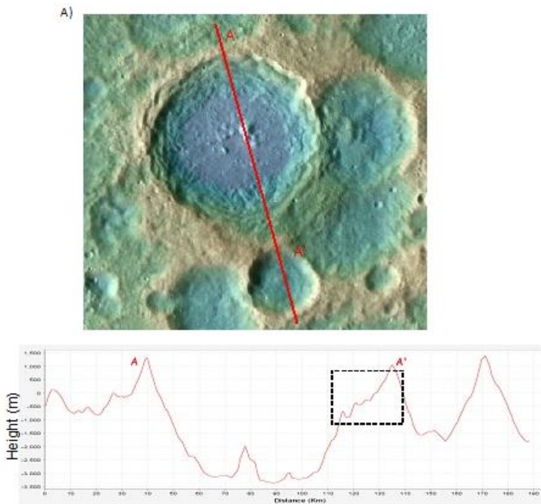
Figure 3.6A: Topography detail of Olcott crater along the NW-SE direction. (Top) LRO LOLA shaded relief map with context view of the profiled area. The topographic expressions of many pre-existing craters are recognizable in this dataset. (Bottom) LRO-LOLA derived topographic profile. The crater walls along the SE part near the crater rim (black box) have greater slumping closer to the rim, different from the NW crater wall. This may be due to the presence of a pre-existing feature that was obliterated during the Olcott forming crater event. [Image credit: MIT/NASA]
