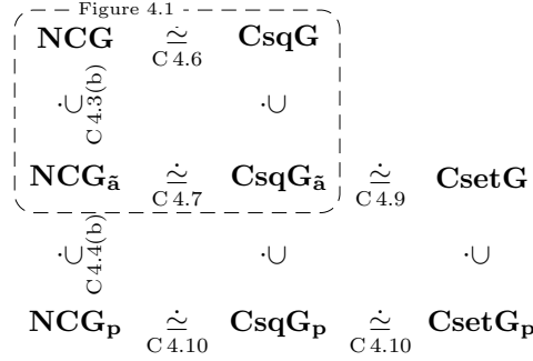
FIGURE 4.2. Some isomorphisms and strict isomorphic inclusions among subcategories of \mathbf{NCG} (C=Corollary).
