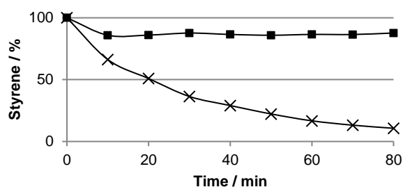
Figure 1. Consumption of styrene ( 1 ) by hydrogenation with WI without additive (x) and with SPN (16 g/mmol Rh) added at the outset of reaction (■). Conversion values were determined by calibrated GC-FID analysis of reaction aliquots with integration relative to an internal standard.
