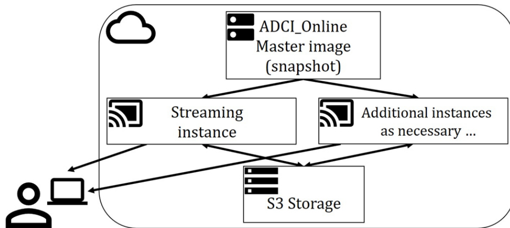
Fig. 1. ADCI Online leverages a cloud-based environment to expand system resources on-demand. All streaming instances are configured identically from an existing snapshot and share the same permanent S3 bucket that contains metaphase images, ADCI outputs and reports. Throughput can be expanded by: (1) cloning system snapshots to provide an array of streaming instances, and/or (2) expanding these computing resources by leasing higher capacity hardware.
