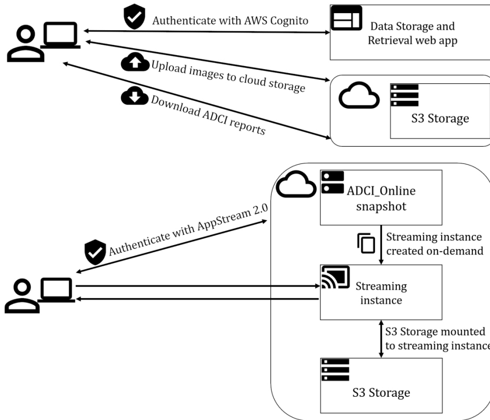
Fig. 2. User interactions with ADCI Online. Top: Once a user validates their AWS Cognito credentials, they sign into the Data Storage and Retrieval web app to upload metaphase images to cloud storage (S3). Bottom: Afterwards, they sign into AWS AppStream 2.0 to request a new ADCI Online streaming session. The user specific S3 folder is mounted to the streaming instance, allowing the user to access their uploaded metaphase images, process samples and save results. Top: After sample processing, dose estimation and report generation, users access and download reports with the Data Storage and Retrieval web app.
