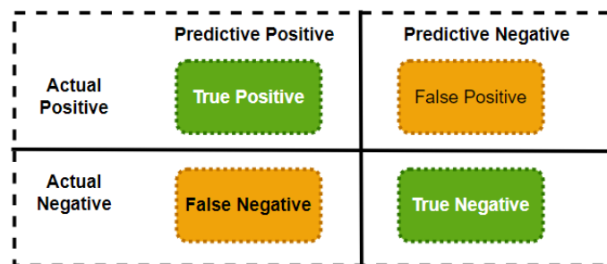
Figure 3.14: Confusion Matrix
