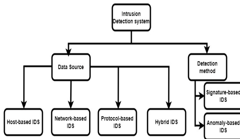
Figure 2.1: IDS Taxonomy
