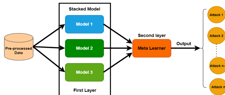
Figure 2.13: Stacking Ensemble Model Architecture
