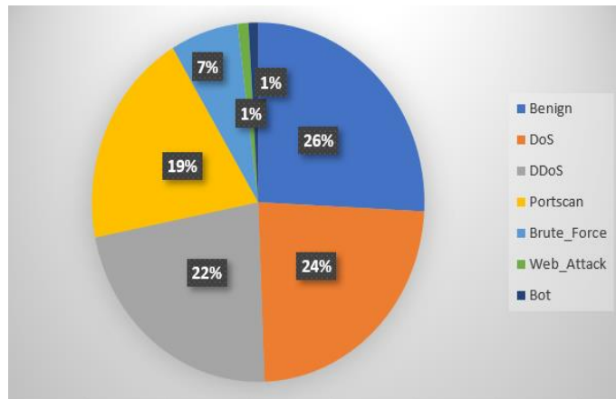
Figure 3.9: CICIDS-2017 Attack Distribution
