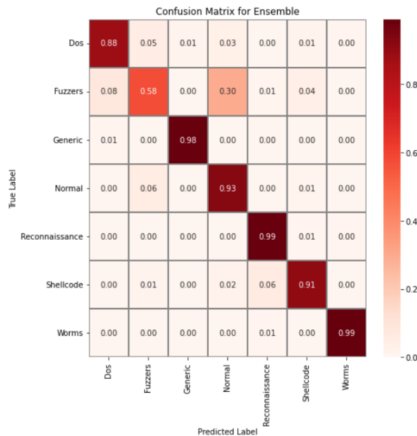
Figure 3.24: Confusion matrix of Ensemble Model
