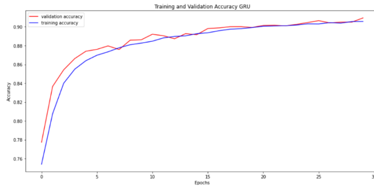
Figure 3.21: Training and validation accuracy of GRU
