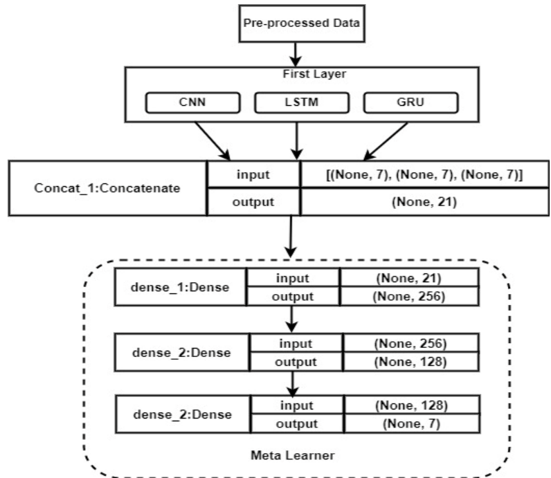
Figure 3.6: Stacking Ensemble System Architecture
