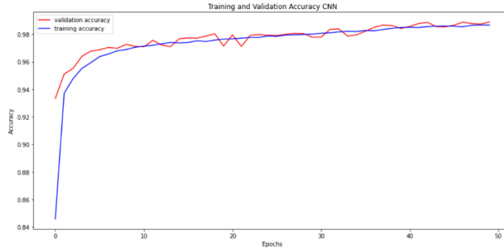
Figure 3.25: Training and validation accuracy of CNN
