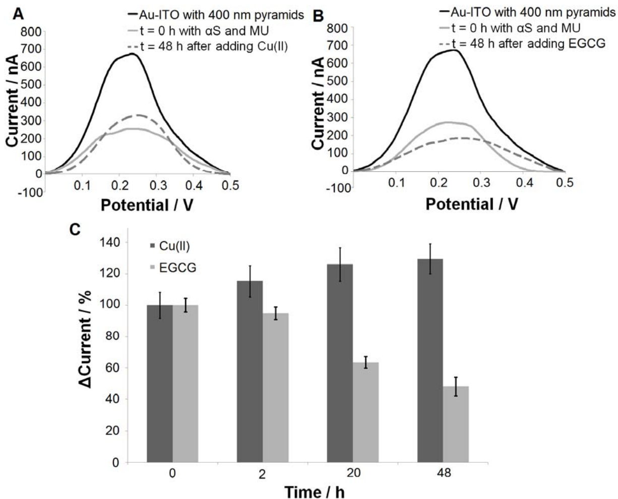
Figure 3 Representative differential pulse voltammograms of \alpha S-immobilized Au-ITO surfaces, displaying the effect of (A) Cu(II) and (B) EGCG incubation on the anodic peak current signals at t = 48 h. (C) Electrochemical analysis of EGCG and metal interactions with \alpha S oligomers showing time dependence study of DPV anodic peak current of 10 mM [\text{Fe}(\text{CN})_6]^{3-/4-} after incubating 50 \mu\text{M} EGCG (light grey) and Cu(II) (dark grey) on corresponding immobilized \alpha S oligomers on Au-ITO surfaces. Other conditions were as described in the experimental section.
