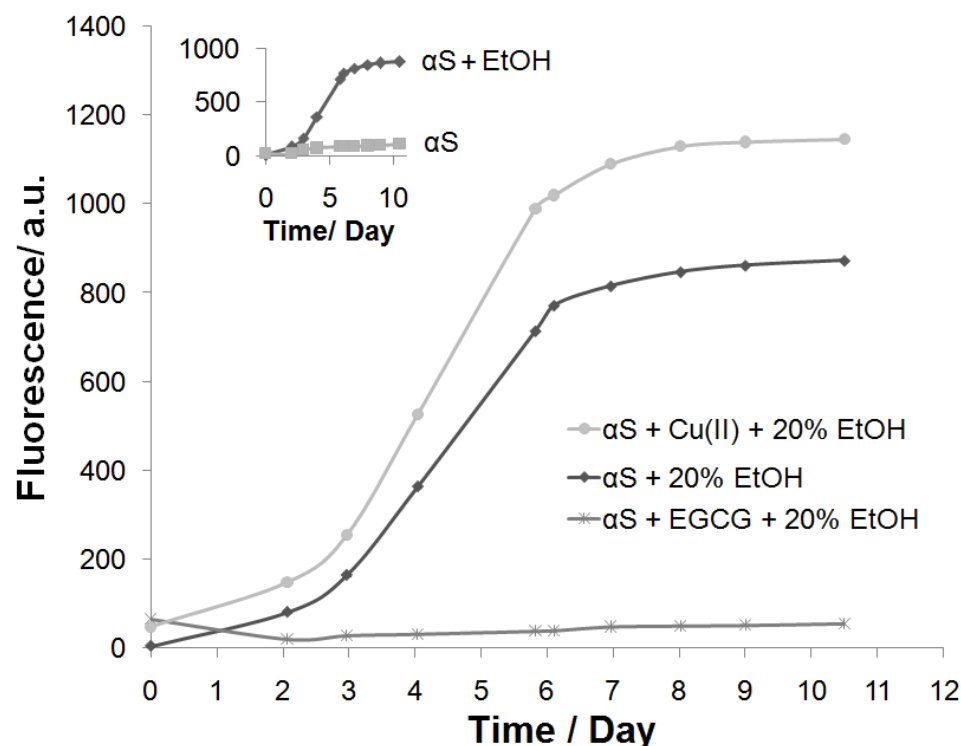
Figure 5. Average relative fluorescence intensity of ThT incubated with 10 \mu\text{M} \alpha\text{S} and 20% ethanol monitored over 10 days in the presence and absence of 50 \mu\text{M} Cu(II) and EGCG. Triplicate measurements were performed for each sample ( n=3 ), and error bars were less than 50 a.u. (not shown). Other conditions were as described in the experimental section.
