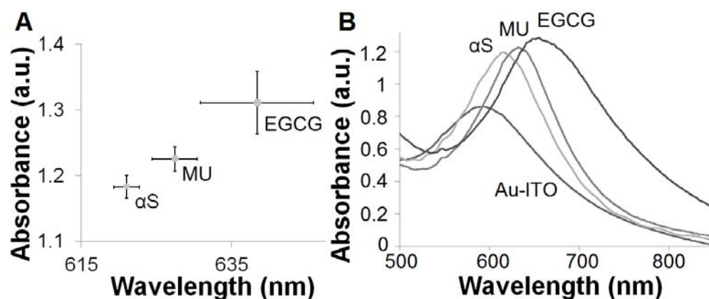
Figure 4. (A) Plot for the variations in LSPR absorption band peak wavelengths and intensities (B) LSPR spectra observed on 400 nm pyramid Au-ITO surfaces as different target biomolecules interacted with \alpha S. Other conditions were as described in the Experimental section.
