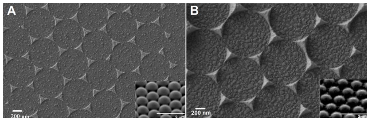
Figure 1. SEM images of (A) Au-nanotriangles and (B) Au-nanopyramids fabricated using NSL at 20,000 X and 30,000 X magnification, respectively. Inset depicts the SEM of nanospheres taken at 45° angle before removal by sonication. Other conditions were as described in the Experimental section.
