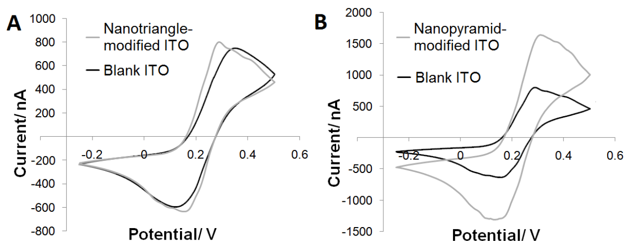
Figure 2. Cyclic voltammograms of 10 mM [\text{Fe}(\text{CN})_6]^{3-/4-} at (A) nanotriangle-modified ITO (grey line) and (B) nanopyramid-modified ITO (grey line) electrodes at a scan rate of 50 mV/s. Black line displays the CV response recorded for the blank ITO electrodes before Au nanostructure modification. Other conditions were as described in the Experimental section.
