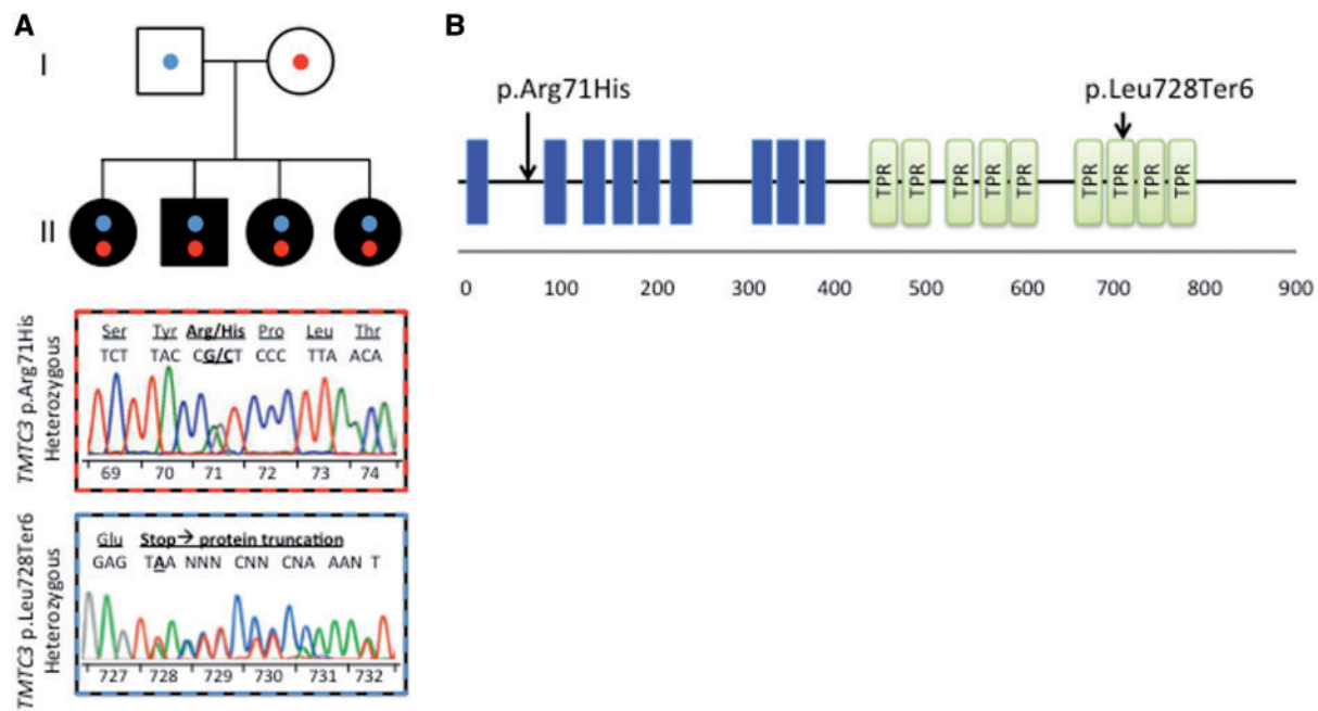
Figure 1. Compound heterozygous TMTC3 variants in patients with nocturnal seizures with developmental delay. (A) Pedigree and electropherograms of the compound heterozygous TMTC3 variants in patients with nocturnal seizures with intellectual disability. Different colored circles in pedigrees represent different variants. (B) Protein structure and associated domains of TMTC3 with respective variants identified. RefSeq numbers: NM_181783.3 and NP_861448.2. Transmembrane regions are shown in blue and the tetratricopeptide repeats (TPR) domains are shown in green. The location of the TMTC3 variants is shown with the black arrows.
