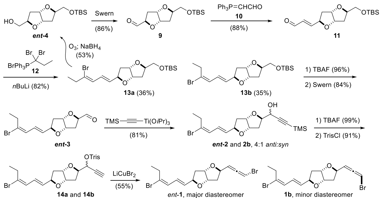
Scheme 3. Synthesis of proposed structure of (+)-aplysallene
