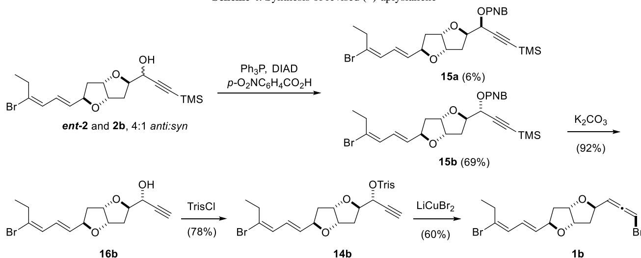
Scheme 4. Synthesis of revised (–)-aplysallene
