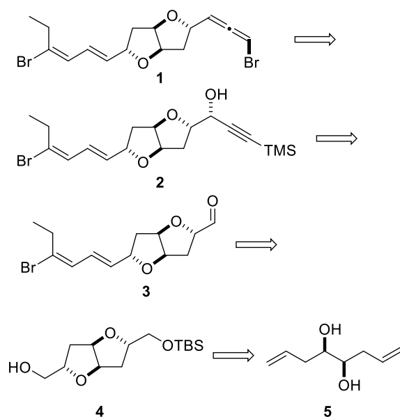
Scheme 1. Retrosynthetic analysis of (-)-aplysiallene.
