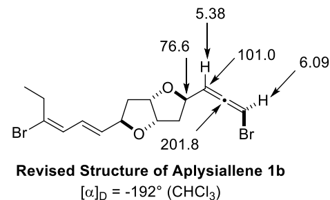
Figure 1. Structural revision of aplysiallene.
