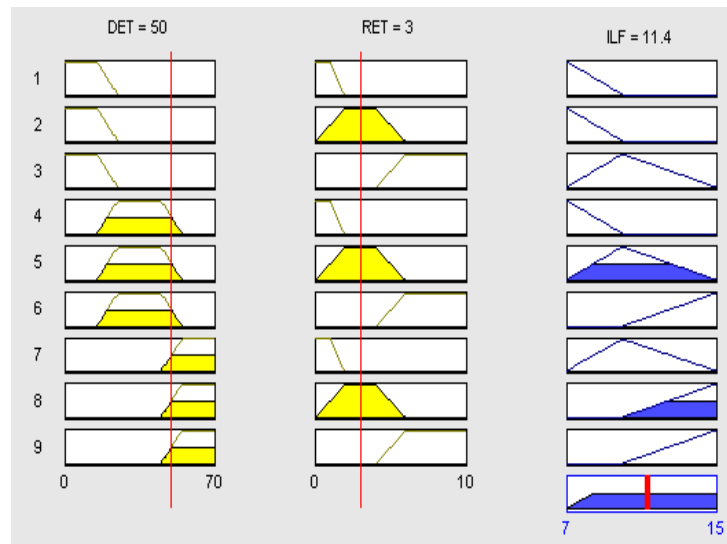
Figure 3: Fuzzy Inference Process of Neuro-Fuzzy Function Points Model
