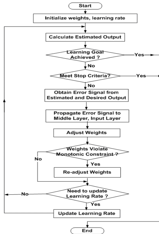
Figure 9: Learning Procedure Flowchart
