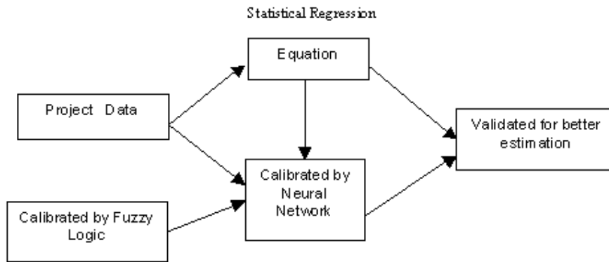
Figure 1: Neuro-Fuzzy Function Points Calibration Model Block Diagram
