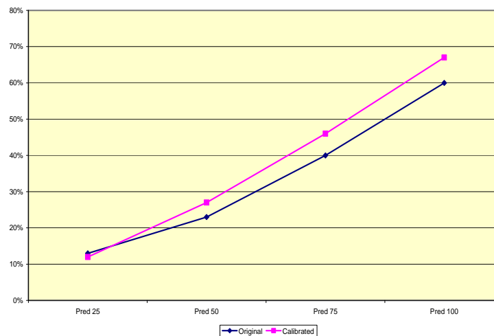
Figure 11: PRED Evaluation Results Comparison
