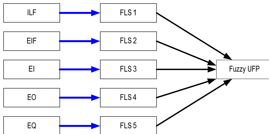
Figure 5: Fuzzy Complexity Measurement System of Neuro-Fuzzy Function Points Model
