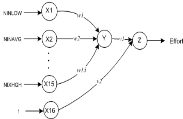
Figure 8: Neural Network Structure
