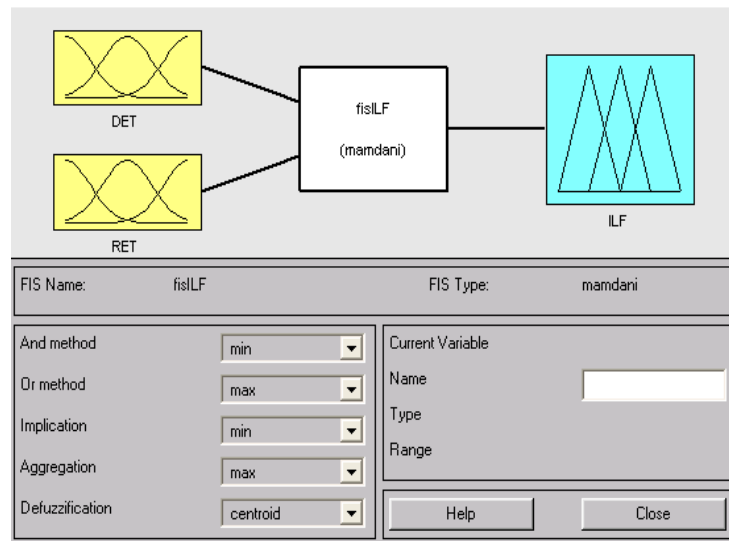
Figure 4: Fuzzy Logic System for ILF
