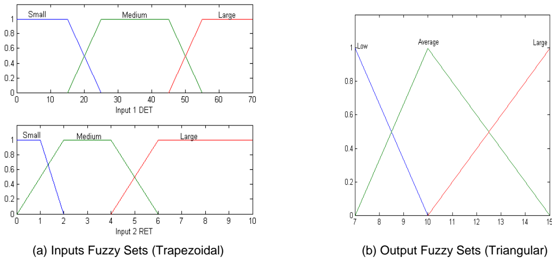
Figure 2: Neuro-Fuzzy Function Points Calibration Model Fuzzy Sets for ILF
