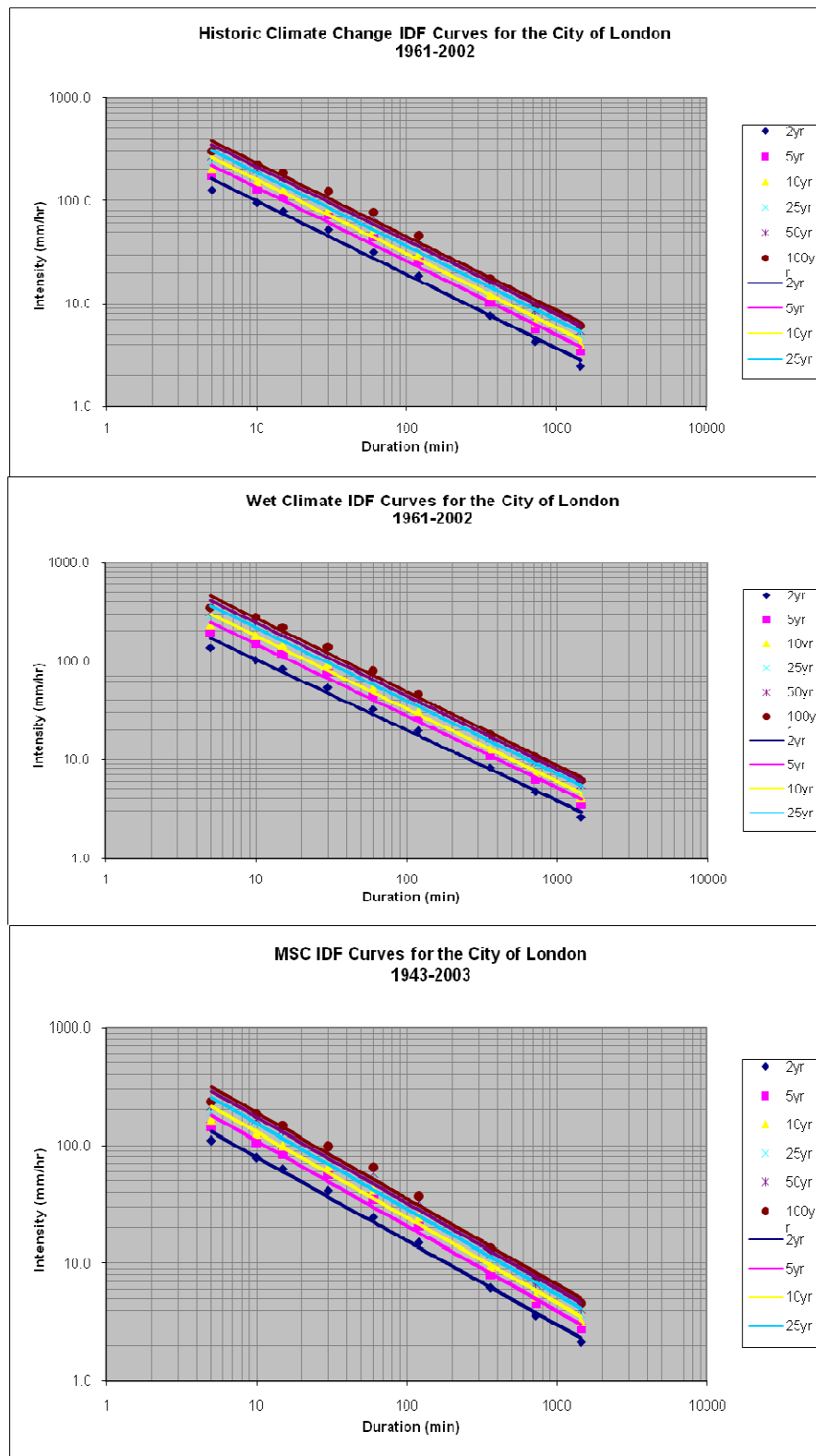
Figure 3. Comparison of IDF curves for the new data set
