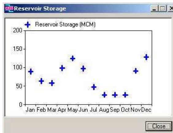
Figure 5.13 Variation of reservoir storage – Type 1
