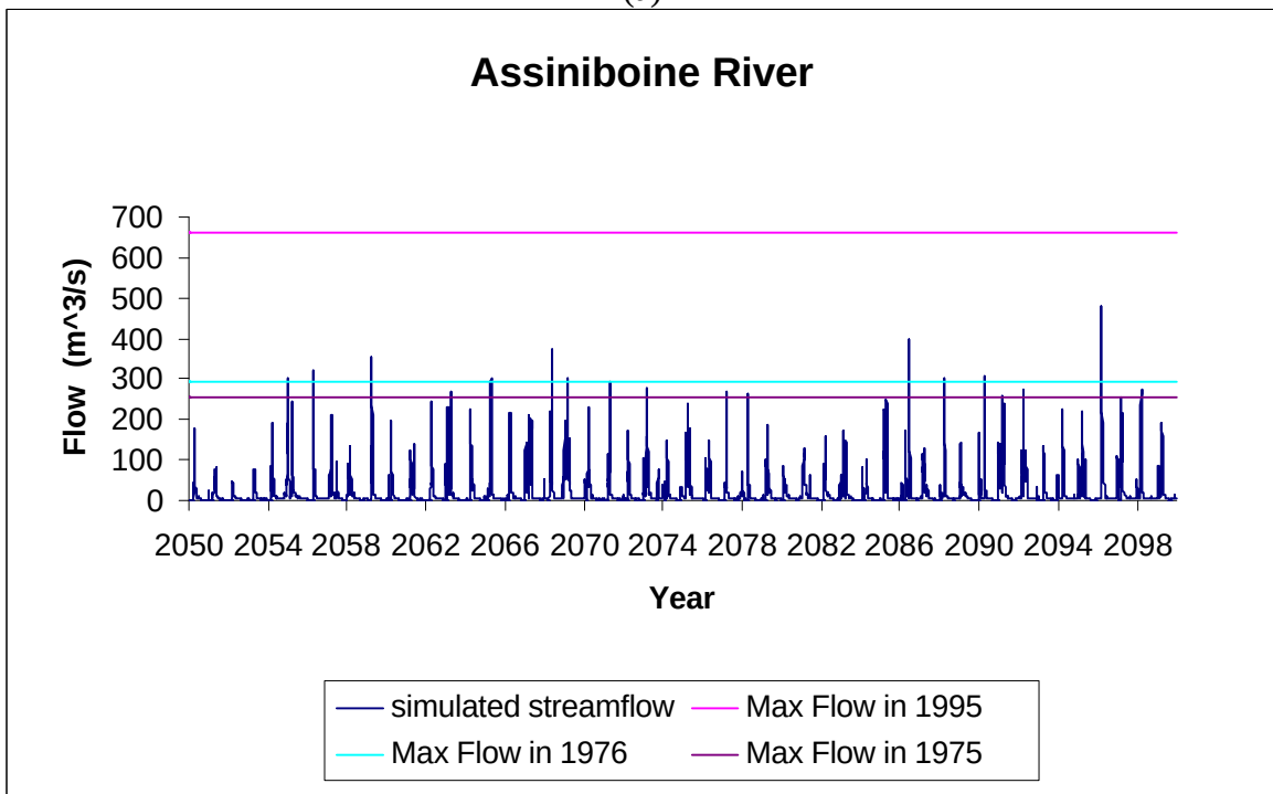
Figure 30. Comparison of the historical data with the simulated streamflow for the scenario 1 of ECHAM4 – Assiniboine River
