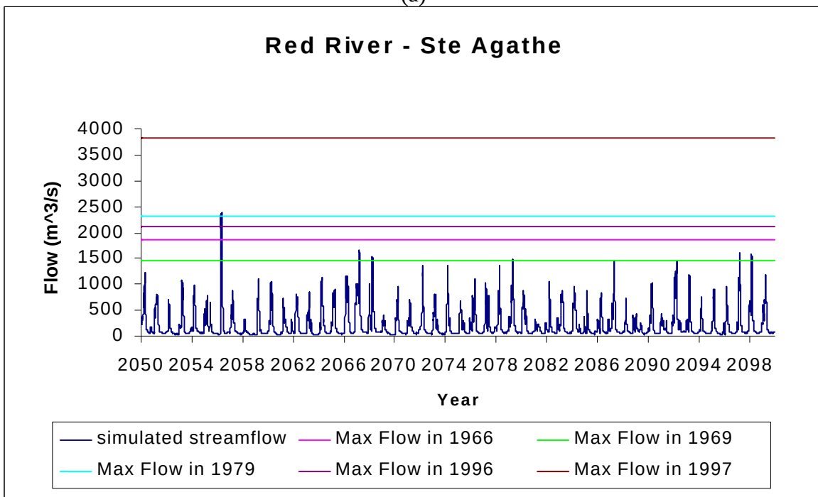
Figure 31. Comparison of the historical data with the simulated streamflow for the scenario 1 of ECHAM4 – Red River at Ste Agathe
