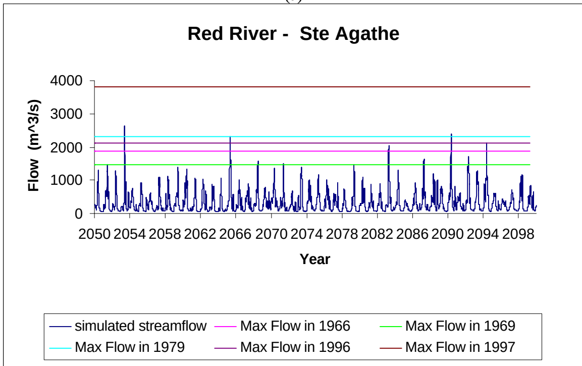
Figure 28. Comparison of the historical data with the simulated streamflow for the scenario 2 of CGCM1 – Red River at Ste Agathe
