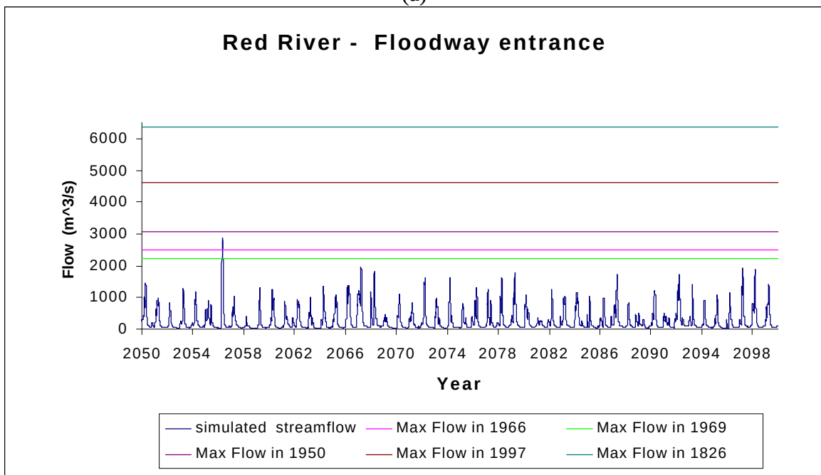
Figure 32. Comparison of the historical data with the simulated streamflow for the scenario 1 of ECHAM4 – Red River at Floodway entrance
