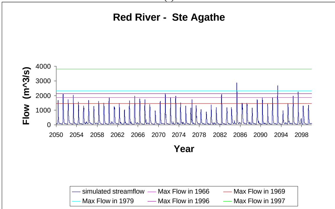
Figure 22. Comparison of the historical data with the simulated streamflow for the control scenario of HADCM3 – Red River at Ste Agathe
