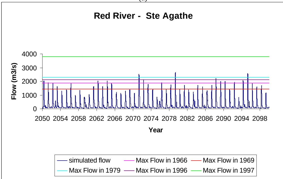
Figure 25. Comparison of the historical data with the simulated streamflow for the scenario 1 of HADCM3 – Red River at Ste Agathe
