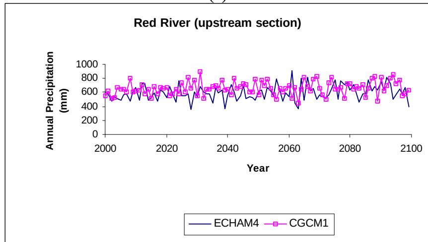
Figure20. Comparison of annual precipitation generated by CGCM1 for scenario S2 and ECHAM4 for scenario S1
