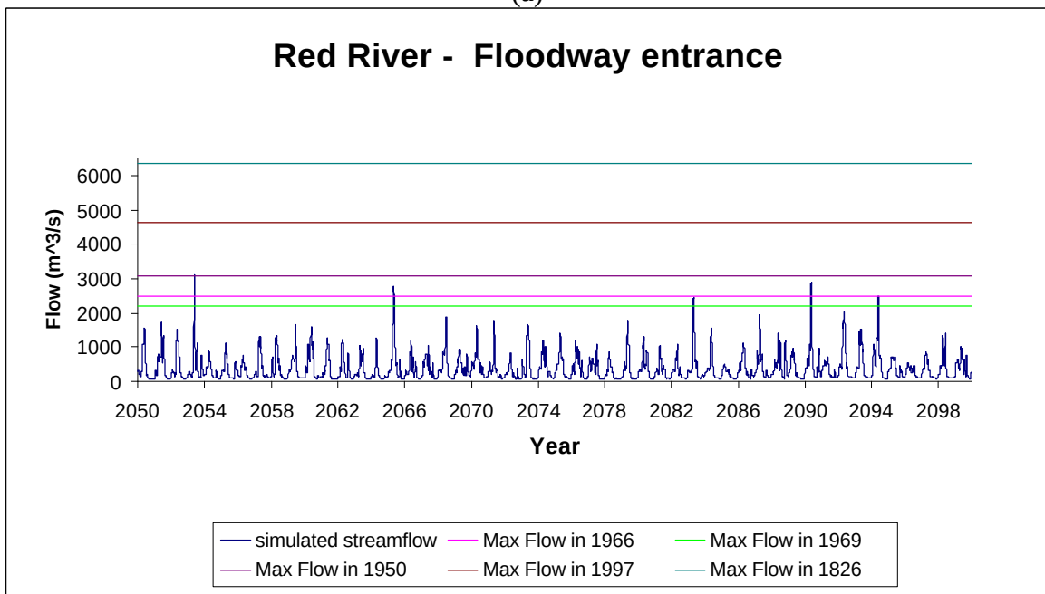
Figure 29. Comparison of the historical data with the simulated streamflow for the scenario 2 of CGCM1 – Red River at Floodway entrance
