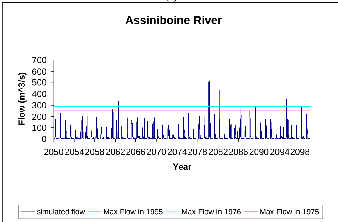
Figure 24. Comparison of the historical data with the simulated streamflow for the scenario 1 of HADCM3 – Assiniboine River
