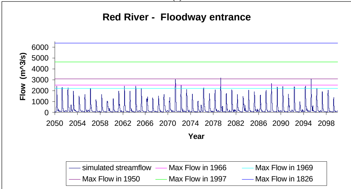
Figure 26. Comparison of the historical data with the simulated streamflow for the scenario 1 of HADCM3 – Red River at Floodway entrance
