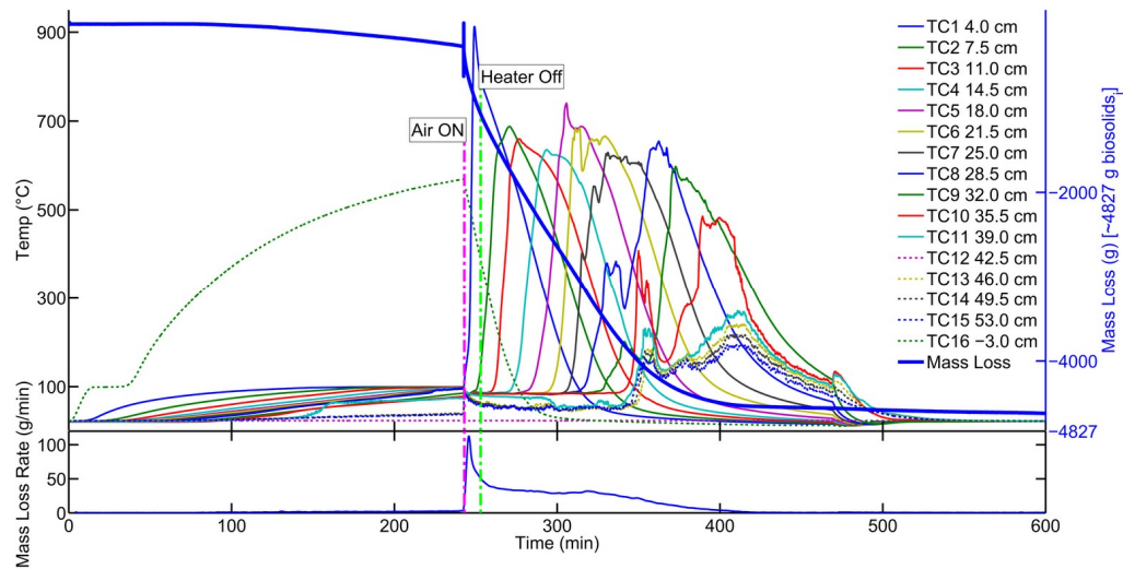
Figure G13: Temperature, mass loss, and mass loss rate profiles for Experiment No. 16, a self-sustaining smouldering experiment with 71% moisture content re-wetted biosolids in a fixed bed at a 1.7 g/g sand/biosolids mass ratio and an air flux of 3.3 cm/s. The solid lines represent thermocouples within the contaminant pack. The top second y axis (blue) shows the initial volatile solids and water mass in the column, 4827 g. The unsteady temperature in TC6 to TC10 is expected to have resulted from water dripping into the reaction front due to the low sand/biosolids mass ratio. Some top sand had been ejected upon air initiation and was corrected in the mass loss data. Due to the ejection, TC11 to 15 were exposed to the atmosphere and represent the air space temperatures above the column upon full combustion. TC12 was broken for this experiment.
