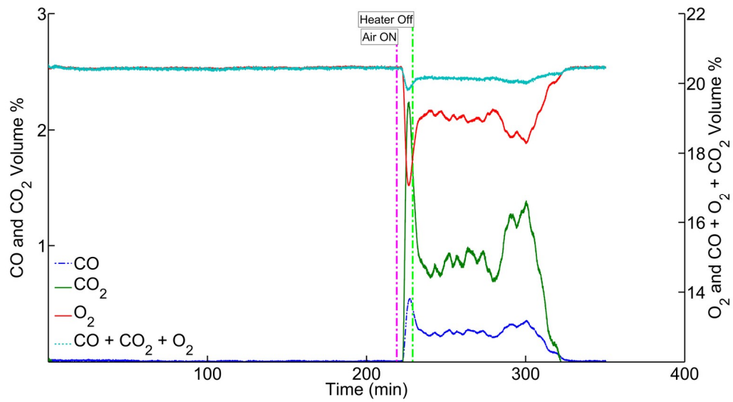
Figure D3: The carbon dioxide ( \text{CO}_2 ) (solid green), carbon monoxide (CO) (dashed blue), oxygen ( \text{O}_2 ) (solid red), and \text{CO}+\text{CO}_2+\text{O}_2 (dotted light blue) volume % for Experiment No. 26.
