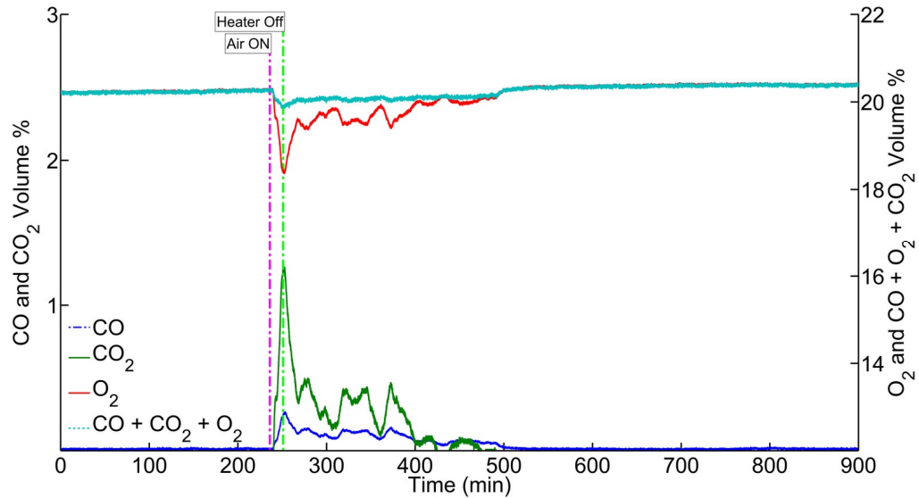
Figure D4: The carbon dioxide ( \text{CO}_2 ) (solid green), carbon monoxide (CO) (dashed blue), oxygen ( \text{O}_2 ) (solid red), and \text{CO}+\text{CO}_2+\text{O}_2 (dotted light blue) volume % for Experiment No. 27.
