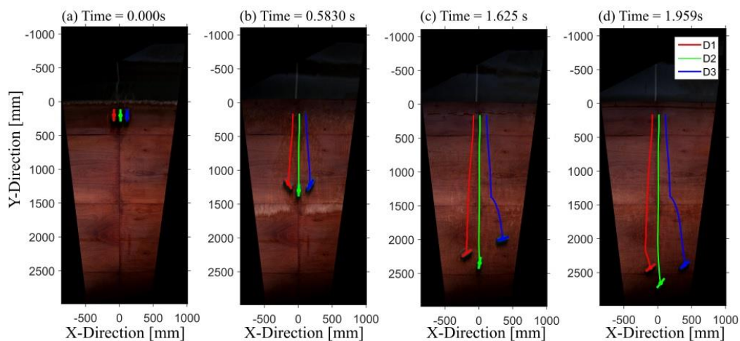
Figure 5: Trajectory of debris (D1 – D3) in experiment #12 (E04) at four instances in time: (a) 0.000 s; (b) 0.5830 s; (c) 1.625 s; (d) 1.959 s.
